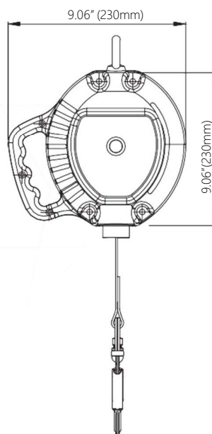
VISTA FRONTAL
